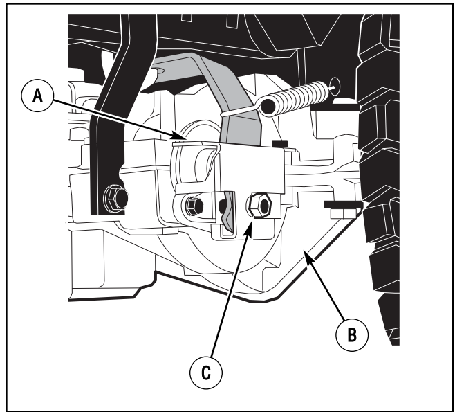
Figure 26: Adjusting drive brake
