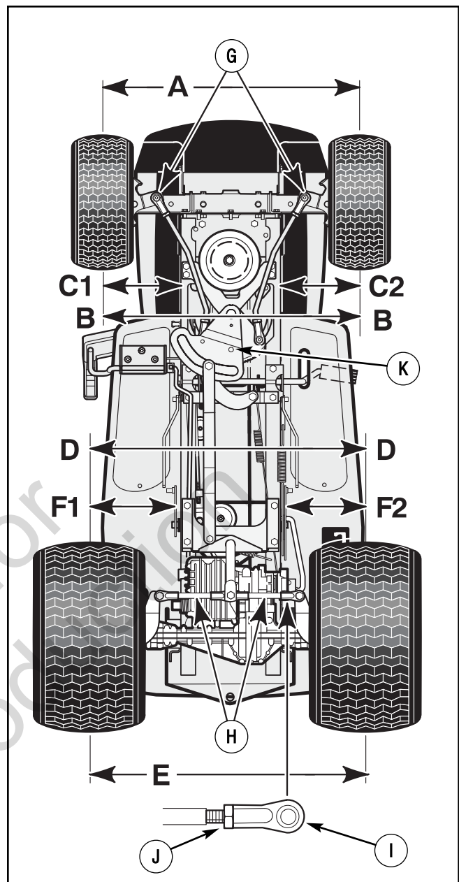
Figure 42: Wheel alignment
